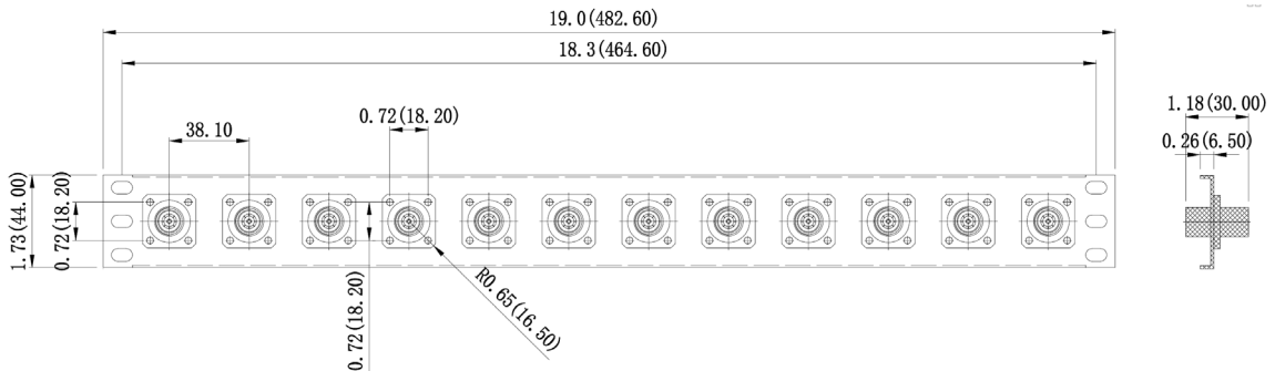
SBH-225-1U : 12x 2.2-5 Female to 2.2-5 Female Adaptors
