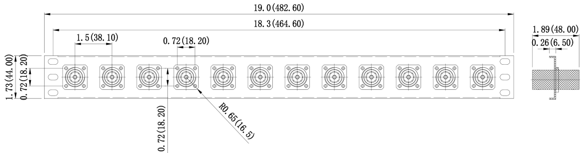
SBH-431-1U : 12x 4.3-10 Female to 4.3-10 Female Adaptors
