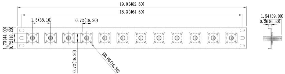
SBH-N10-1U : 12x NEX10 Female to NEX10 Female Adaptors
